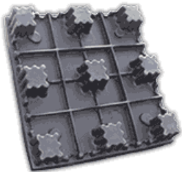
Underside view shows the truss-designed steel frame running both directions to provide rigid stability and strength.
